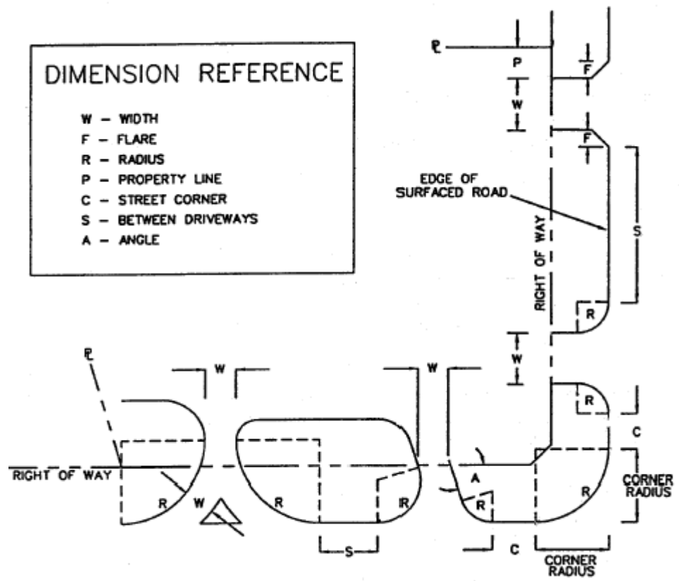
FIGURE 7.3 DRIVEWAY DESIGN STANDARDS
